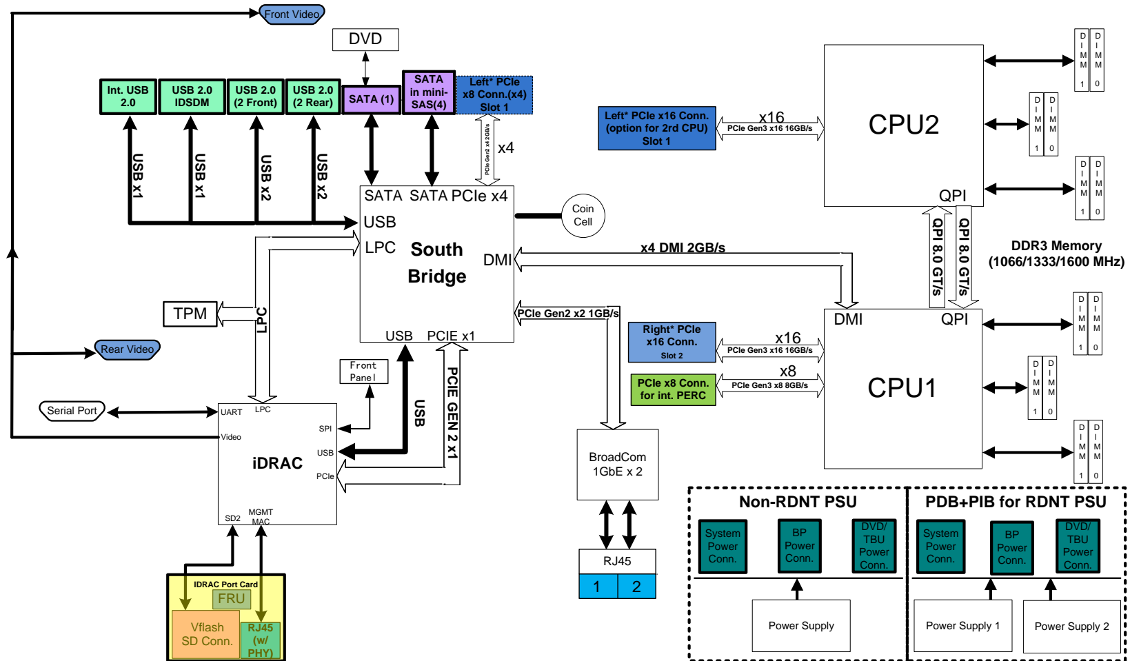
Figure 13. R420 system board block diagram
