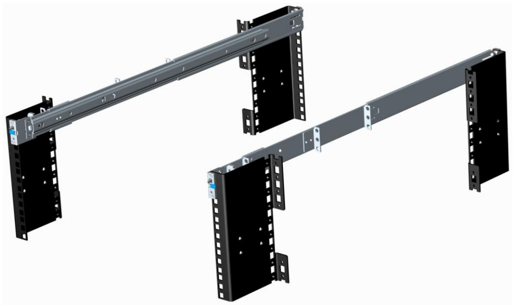
Figure 9. Static rails
